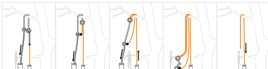
Fig.14 - A rope can be installed directly from below through the use of a cambium saver and a cord. This allows the worker to ascend the rope quickly and safely. At the end of the operation, it is possible to remove the rope and the cambium saver from the ground.
