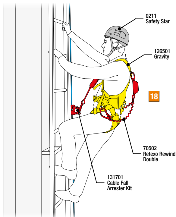
Fig.18 - Vertical metal structures (such as cableway pylons and wind farm turbine poles) are often equipped with ladders for progression combined with a vertical anchoring cable on which fall arrest devices can be installed. These devices are designed to follow the operator during movement and intervene to arrest any fall.
