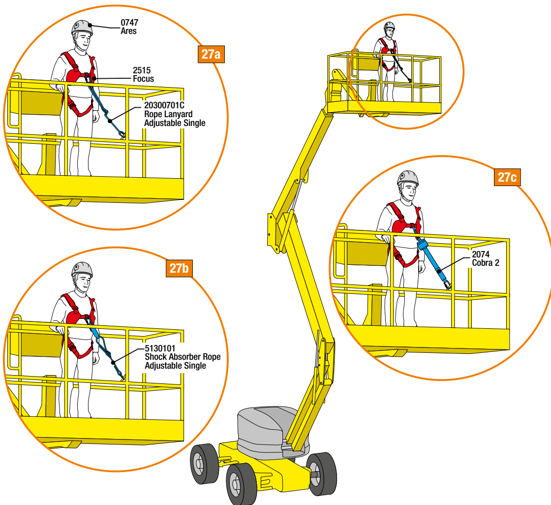
Fig.27 - The simplest solution for preventing the risk of the operator being thrown from the platform is by using a full body harness to which an adjustable positioning lanyard is secured. By securing this to the appropriate anchoring points on the platform and appropriately adjusting the length, the operator will remain anchored to the surface of the platform even in the event of dangerous vertical oscillations ( fig.27a ). Should the risk of falling off the platform persist, the use of an adjustable lanyard with an energy absorber ( fig.27b ) or a retractable fall arrester must be evaluated ( fig.27c ).
