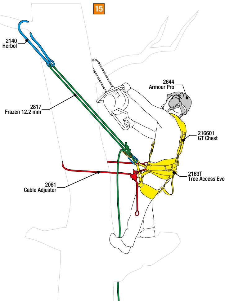
Fig.15 - The choice between various operational techniques must be made taking into consideration the peculiarities that are present in the large range of situations that may occur while working in trees. During cutting operations, the use of equipment that is designed to be the most resistant to chainsaw cutting is essential (i.e. positioning lanyard with steel core). For maximum freedom of lateral movement, a harness with a mobile ventral attachment system is used.
