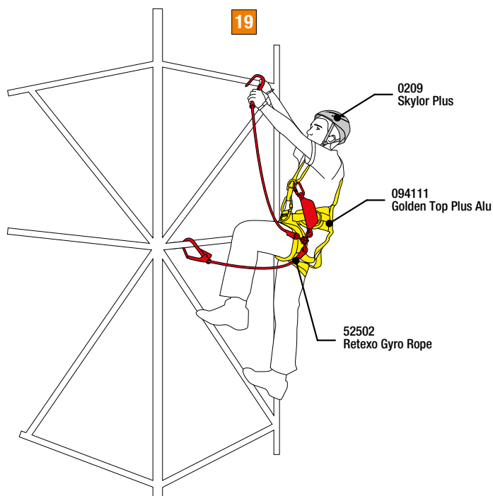
Fig.19 - For progression on structures without anchoring systems, the operator can proceed by anchoring himself directly to the structure (after verifying its strength) by means of a double lanyard with energy absorber and connectors suitable for the size of the structure.
